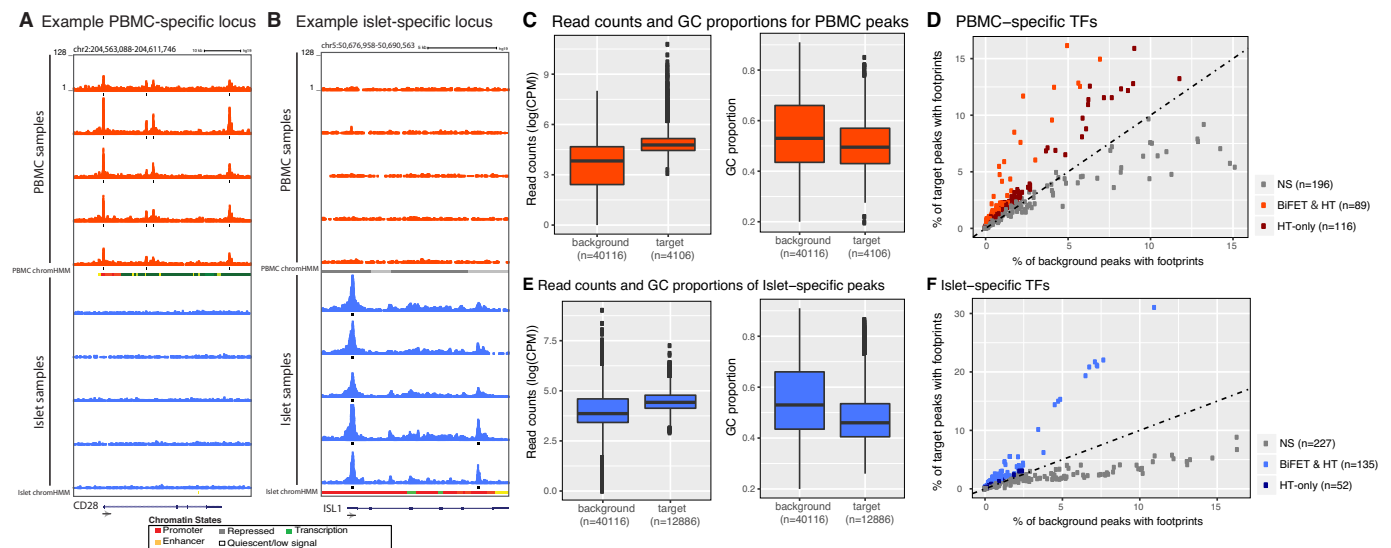
Figure 3. Footprints enriched in PBMC and islet-specific ATAC-seq peaks. (A) UCSC genome browser track for example PBMC-specific peaks located around the CD28 locus. Chromatin accessibility maps in PBMCs (islets) are shown in red (blue). ChromHMM (41) states for PBMCs and islets are represented as colored bars. All genome browser sessions are normalized to the same scale. The labels for scales are omitted from some panels for readability. (B) Example islet-specific peak located around the promoter of ISL1 . (C) Read counts (left panel) and GC content (right panel) of PBMC-specific (target) peaks versus background peaks in PBMC samples. (D) Percent of target peaks with footprints versus percent of background peaks with footprints for each TF in PBMC samples. The TFs that are significant by both BiFET and HT are labeled 'BiFET & HT' and indicated by red dots, those that are significant only by the HT ('HT-only') are colored in dark red, and the TFs that are not significant ('NS') by either method are colored in gray. (E) Read counts (left panel) and GC contents (right panel) of islet-specific (target) peaks versus background peaks in islet samples. (F) Percent of target peaks with footprints versus percent of background peaks with footprints for each TF in islet samples. The TFs that are significant by both BiFET and HT are labeled 'BiFET & HT' and colored in blue, those that are significant only by the HT ('HT-only') are colored in dark blue and the TFs that are not significant ('NS') by either method are colored in gray.
